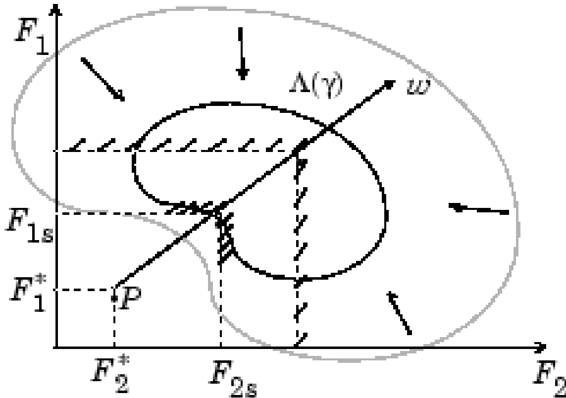
Figure 7-1, Geometrical Representation of the Goal Attainment Method
